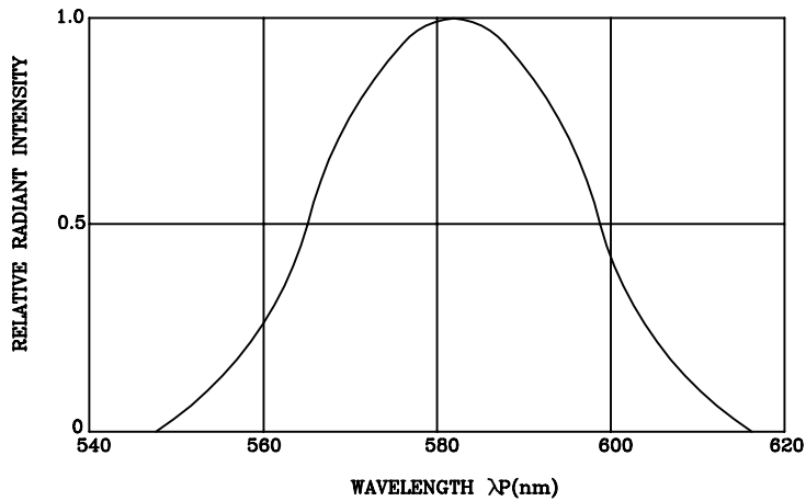
SPECTRAL DISTRIBUTION
