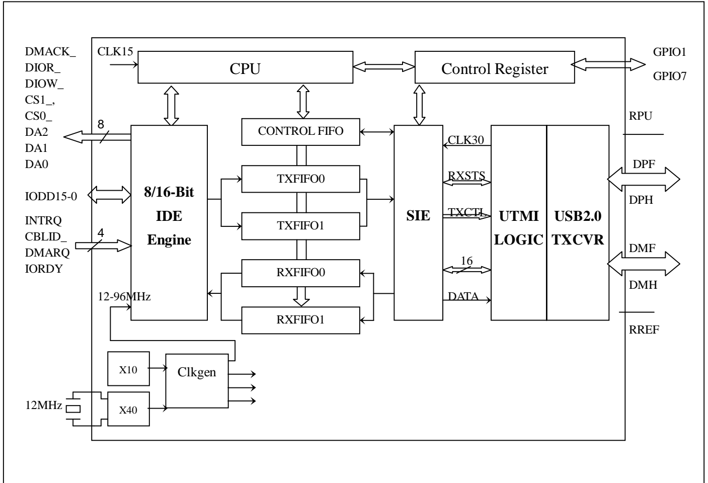
Figure 4.1 - Block Diagram
